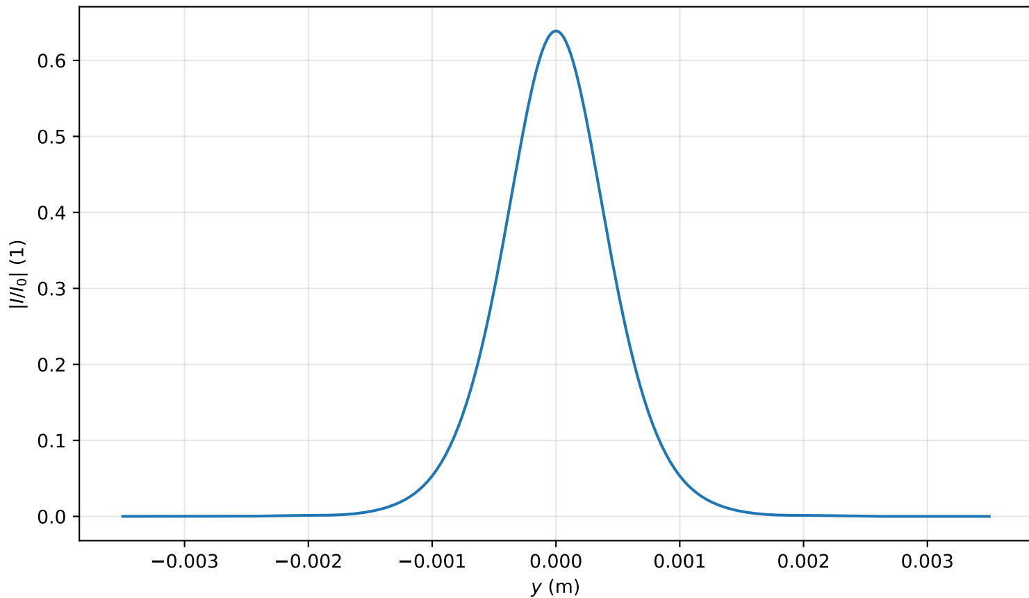
Intensity profile I(x=0, y, z=3.901)/I_0 , P_{in}=0.7P_{cr} , artificial time
